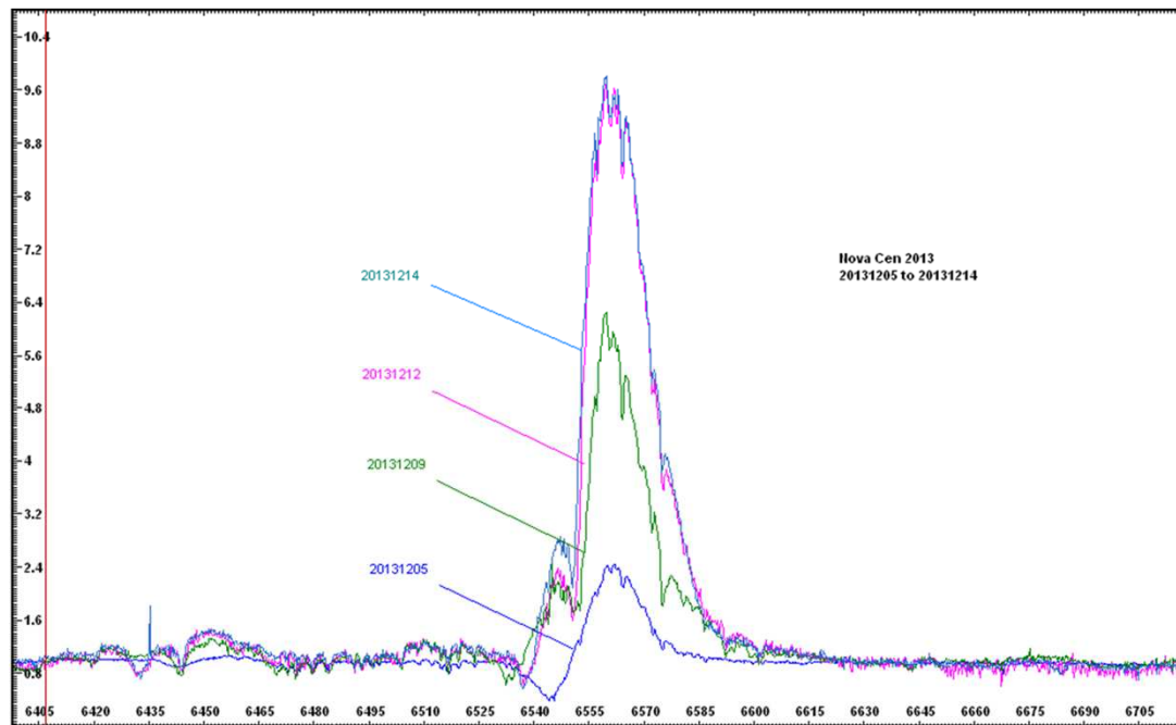
H-Alpha na Nova Centauri 2013 (20131205 a 20131214)
